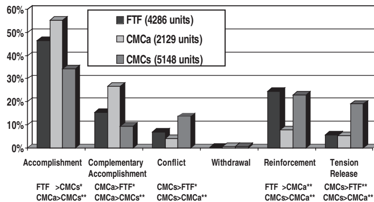
Figure 2: Mean Percentage of the Six Interaction Categories in the Three Communication Modalities
